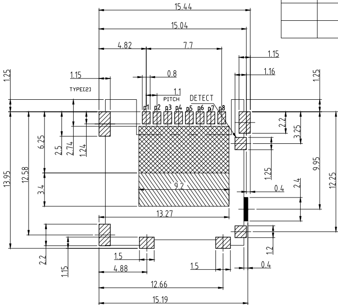
RECOMMENDED PCB PATTERN LAYOUT(TOP VIEW) TOLERANCE: ±0.05
