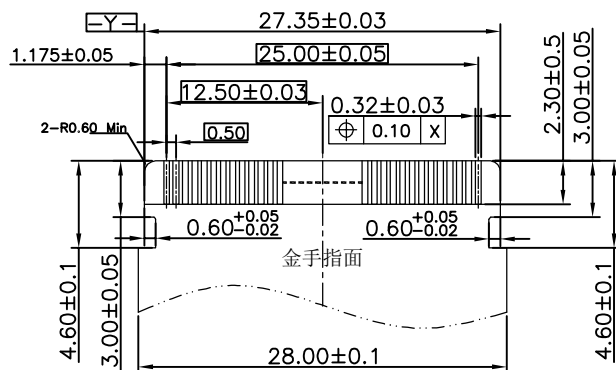
APPLICABLE FPC RECOMMENDED DIMENSION 一体补强板铝箔FPC线(接地)
