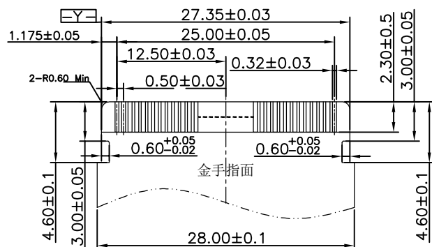
APPLICABLE FPC RECOMMENDED DIMENSION 蓝白裸线(不接地)
