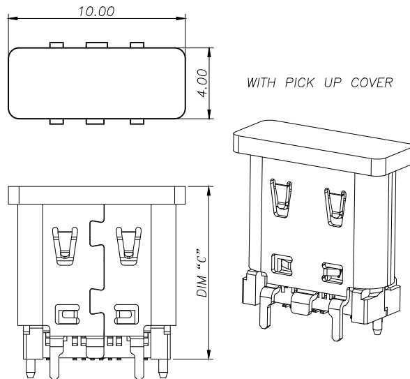
ASSEMBLY WITH CAP
