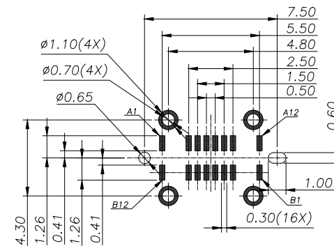
RECOMMENDED PCB LAYOUT(TOP VIEW) THICKNESS 1.0±0.10MM;DEFAULT TOLERANCE:±0.05
