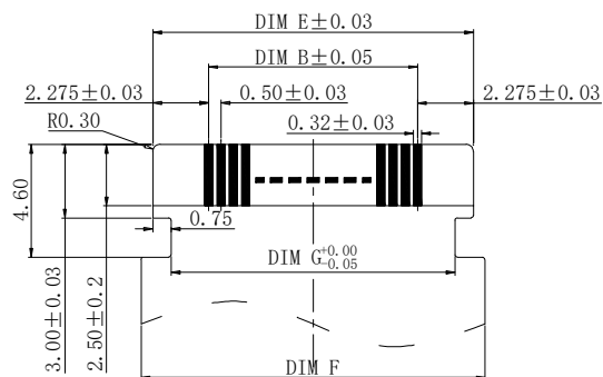
APPLICABLE FPC RECOMMENDED DIMENSION 蓝白裸线(不接地)
