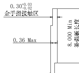
APPLICABLE FPC RECOMMENDED DIMENSION 蓝白裸线(不接地)
