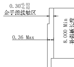
APPLICABLE FPC RECOMMENDED DIMENSION 一体补强板铝箔FPC线
