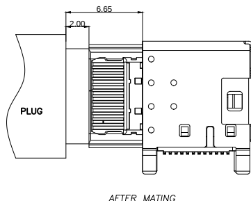
AFTER MATING
