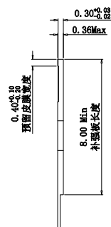
APPLICABLE FPC RECOMMENDED DIMENSION 一体补强板铝箔FFC线(接地)
