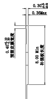
APPLICABLE FPC RECOMMENDED DIMENSION 蓝白裸线(不接地)
