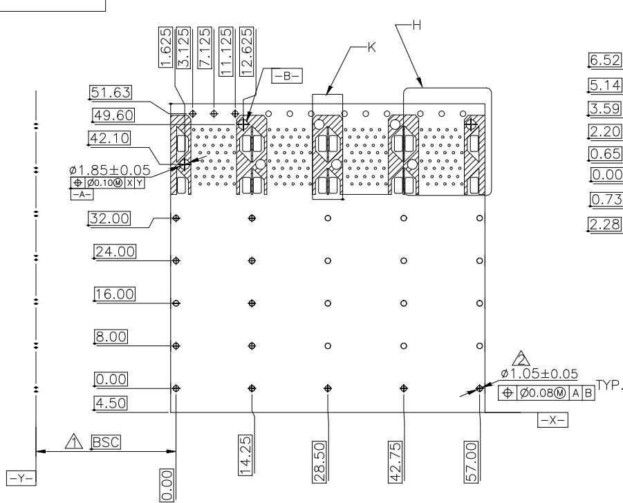
RECOMMENDED PCB CONFIGURATION
