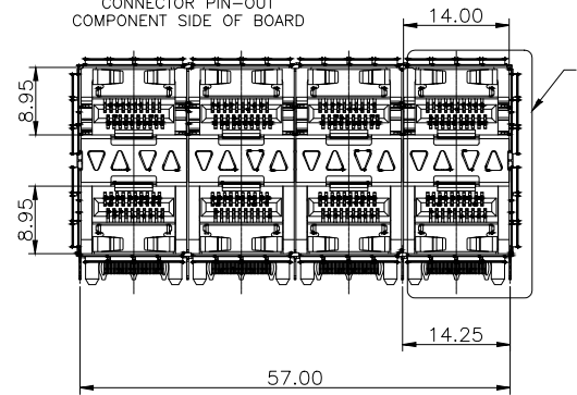
CONNECTOR PIN-OUT COMPONENT SIDE OF BOARD
