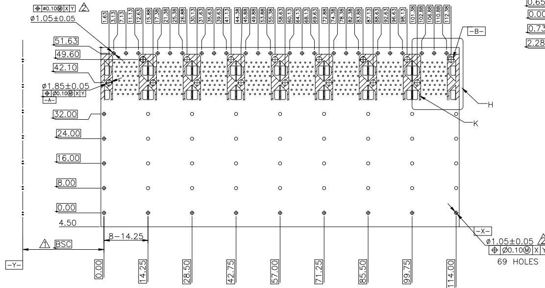
RECOMMENDED PCB CONFIGURATION
