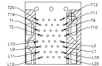
CONNECTOR PIN-OUT COMPONENT SIDE OF BOARD
