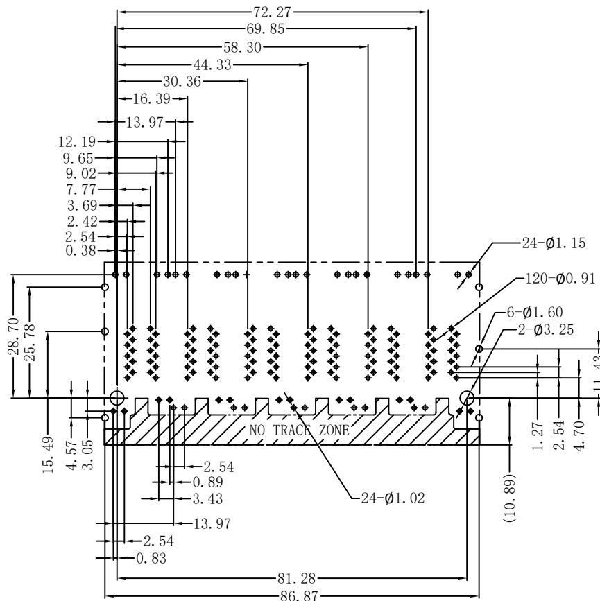
SUGGESTED PCB BOARD LAYOUT VIEWED FROM COMPONENT SIDE
