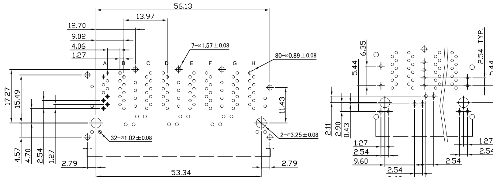
RECOMMENDED PCB LAYOUT (COMPONENT SIDE VIEW)
