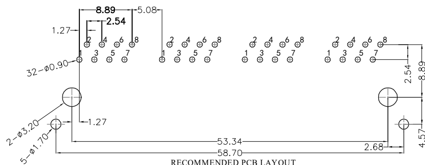
RECOMMENDED PCB LAYOUT VIEWED FROM COMPONENT SIDE
