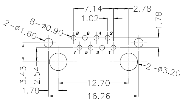
RECOMMENDED PCB LAYOUT VIEWED FROM COMPONENT SIDE
