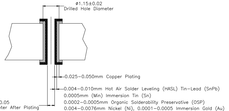
FINISHED HOLE SIZE SPECS
