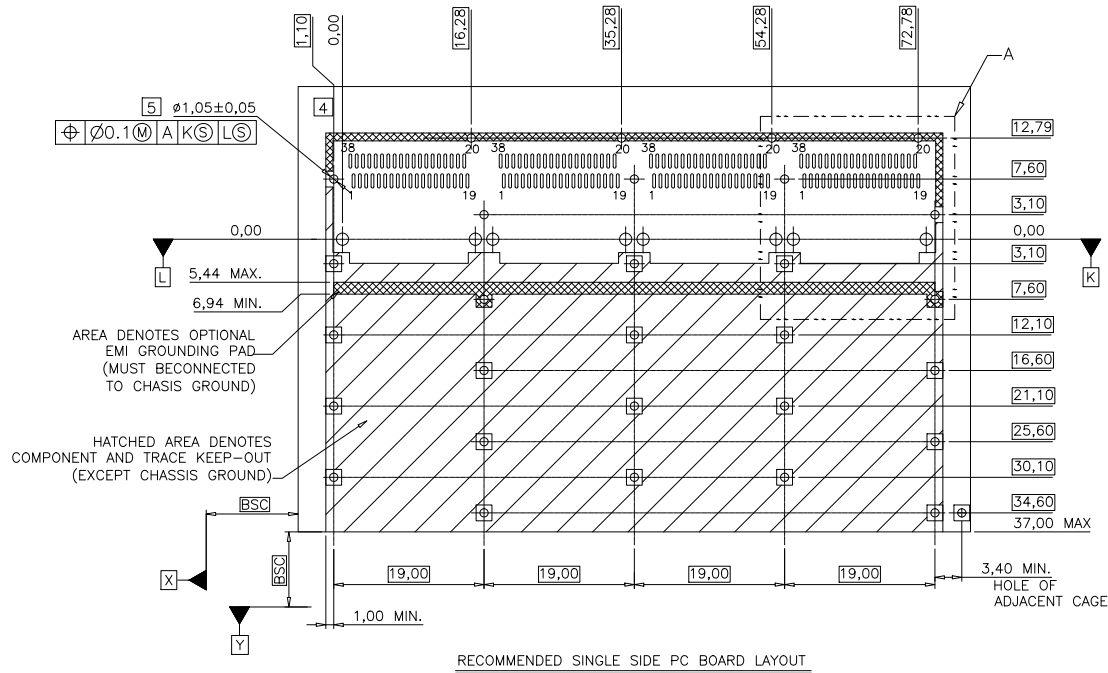
RECOMMENDED SINGLE SIDE PC BOARD LAYOUT
